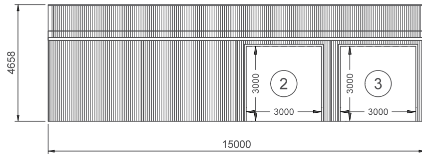
1 SIDEWALL A BUILDING ELEVATION 2 SCALE: 1:150
