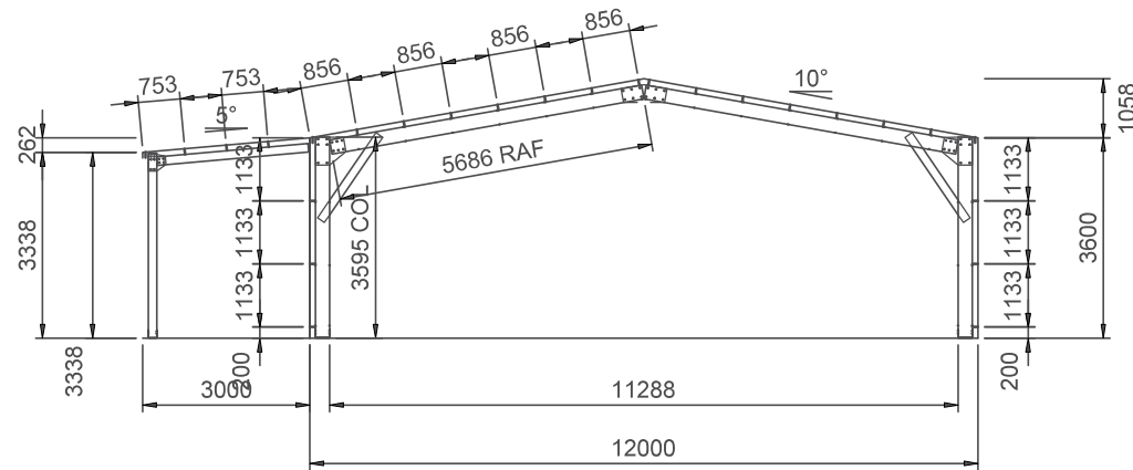
5 INTERNAL FRAMING ELEVATION 2 SCALE: 1:150 FRAMES 2-4
