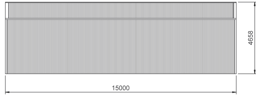
2 SIDEWALL B BUILDING ELEVATION 2 SCALE: 1:150
