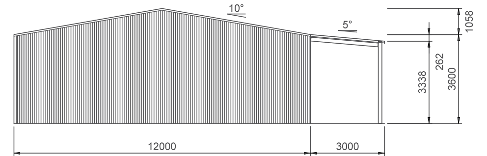
4 FRONT BUILDING ELEVATION 2 SCALE: 1:150 FRAME #1
