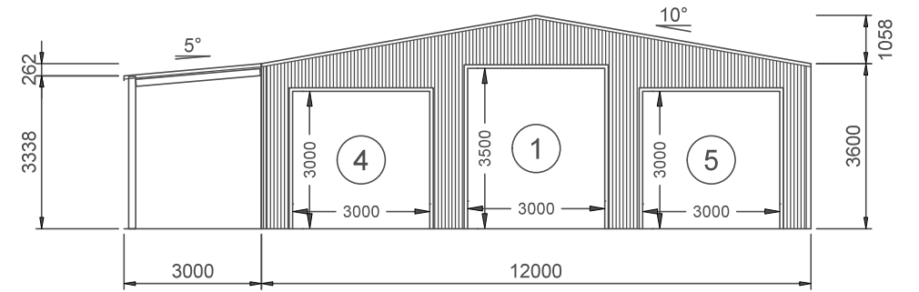
3 REAR BUILDING ELEVATION 2 SCALE: 1:150 FRAME #5
